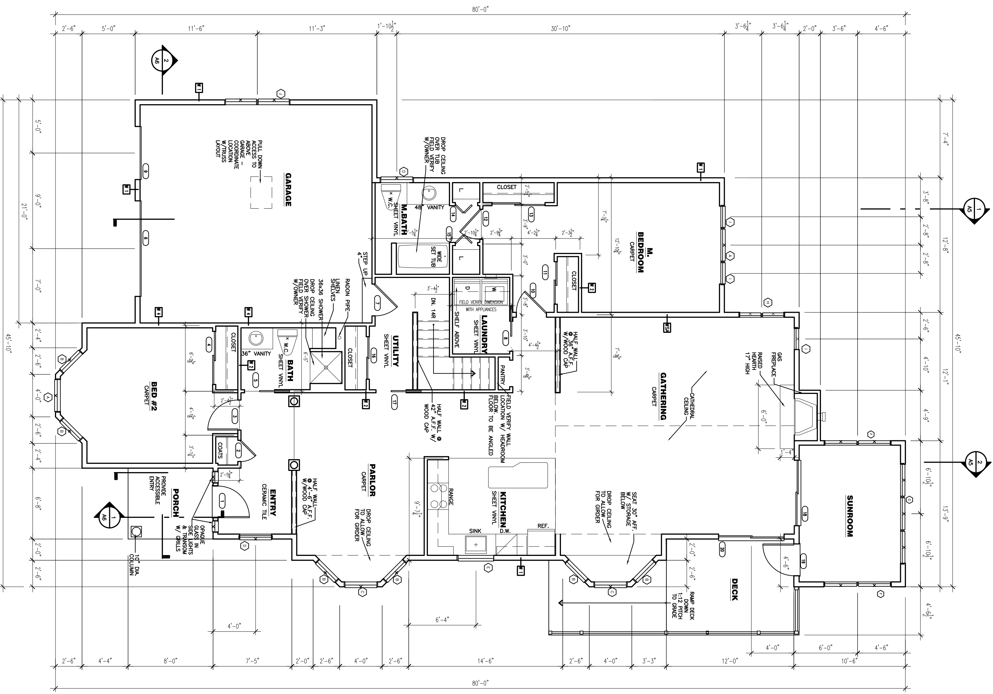
FIRST FLOOR PLAN (UNIT D) 2,010 S.F. SCALE: 3/16"=1'-0"
